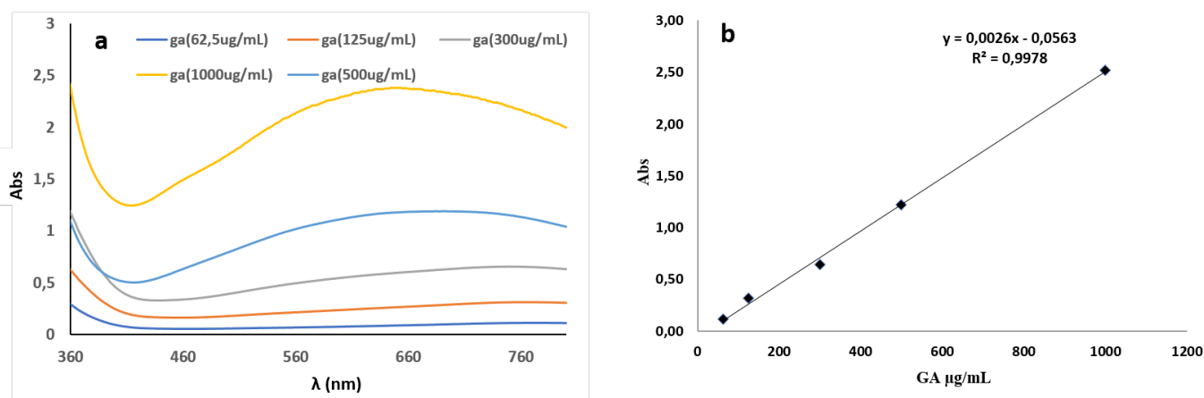
Figure 1. (a) Absorption spectra of GA at different concentrations and (b) GA calibration curve
