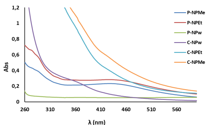
Figure 2. Spectra of AgNPs synthesized from C. Spinosa and P. laurocerasus extracts in DMSO
